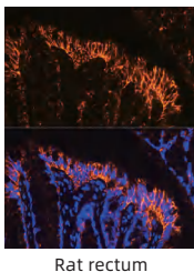
Rat rectum
