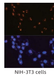
NIH-3T3 cells
