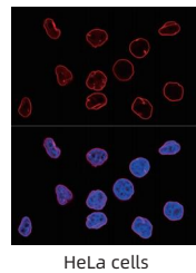
HeLa cells
